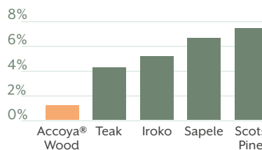
Accoya TRADA shrinkage test
