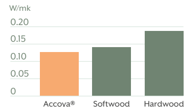
Accoya thermal conductivity test
